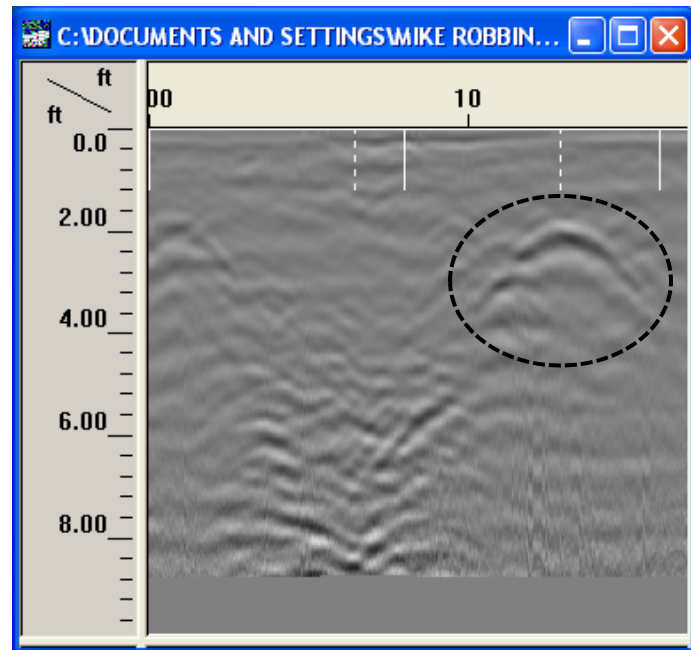
GPR Transect 545 East Across UST
